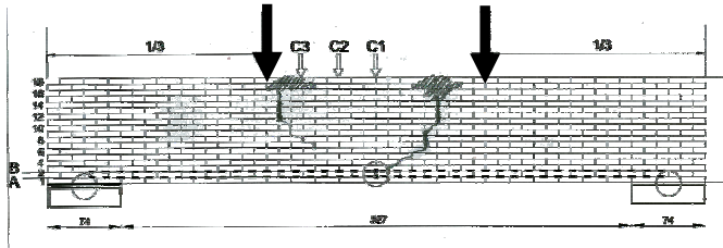
Figure 19. Failure due to horizontal compression of the 1 st tested brick lintel (2 inox. B 800). Figure 20. View of collapsed brickwork after testing: a) At the left jack; b) At the right jack.
