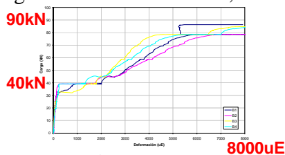
Figure 21: 1 st Test: a) Stress-strain diagram of extensometric gauges (B1, B2, B3, B4) set on reinforcement; b) Readings of the vertical displacement load recorded by LVDTs (C1, C2, C3).
