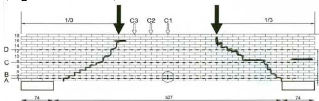
Figure 22. Type of shear failure of the 2 nd tested brick lintel (4 Inox. B 800). Figure 23. View of collapsed lintel after testing: a) left shear crack; b) right shear crack.
