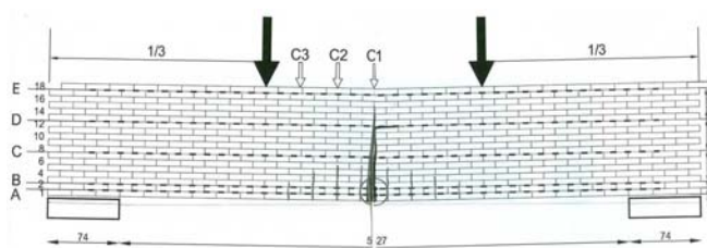
Figure 24. Shear failure of the 3 rd tested brick lintel (5 galva. B 500). Figure 25. View of collapsed lintel after testing: a) central crack; b) reinforcement detail.
