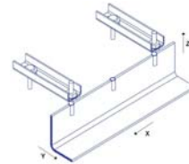
Figure 2. Standard European brackets anchored to a rail, embedded in the face of the slab.
