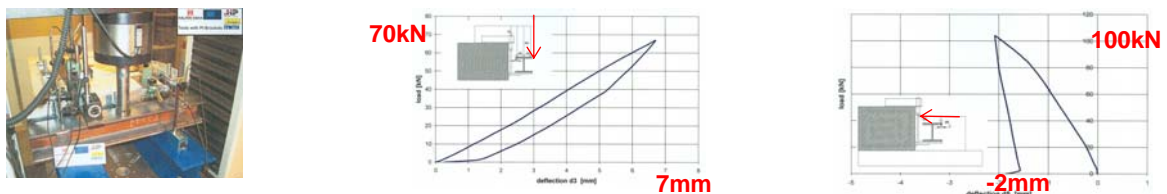
Figure. 9. Testing of one of the three Halfen-AllWall Pi-Bracket prototypes in Germany.
