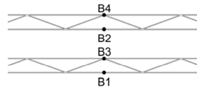
Figure 11. a) Continuous bed joint reinforcement; b) Murfor.5/S-80mm. 5.85m (inox. B800) Figure 12: Arrangement of extensometric gauges in 2 Murfor centre (B1, B2, B3, B4).
