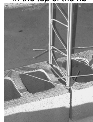
Concrete hollow block + Murfor + AllWall Ribs
